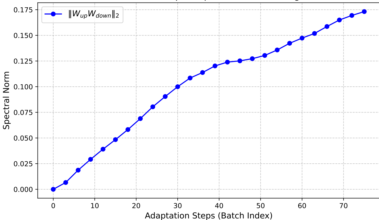
Evolution of Adapter Spectral Norm during TTA
